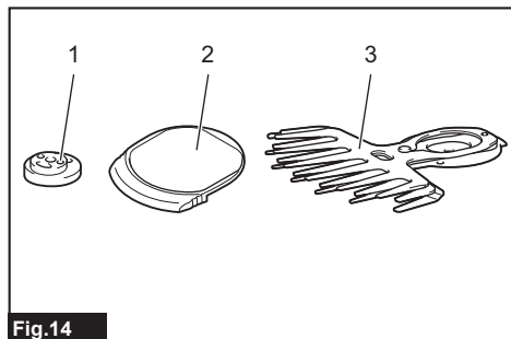
► 1. Crank 2. Undercover 3. Grass shear blades
