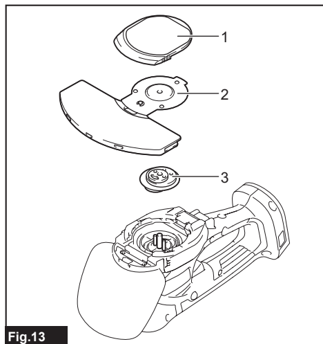
► 1. Undercover 2. Grass shear blades 3. Crank
